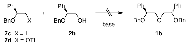
Scheme 4 Ether 1b can not be synthesized from electrophiles 7c and 7d with alcoholate derived from 2b .
